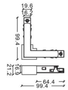
T- connector - R
