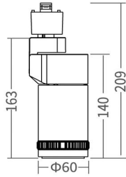
3-pin track adaptor
