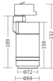
4-pin track adaptor
