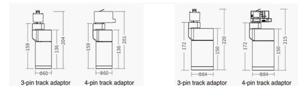
3-pin track adaptor
