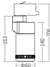
4-pin track adaptor
