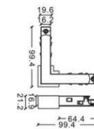
T- connector - R
