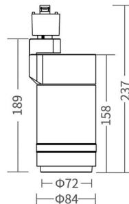
3-pin track adaptor
