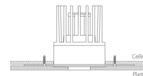
Installation diagram
