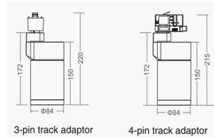
3-pin track adaptor
