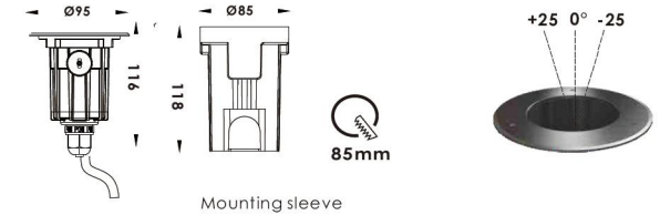
Mounting sleeve
