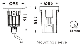
Mounting sleeve
