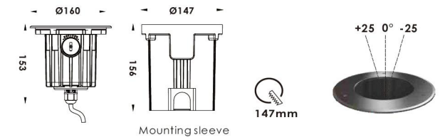
Mounting sleeve
